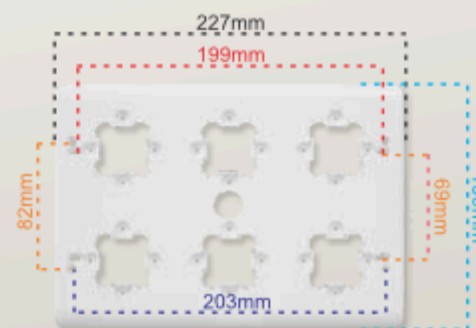
COVER FRAME FOR 6 MODULE SUITABLE FOR 8"X6" FRAME
