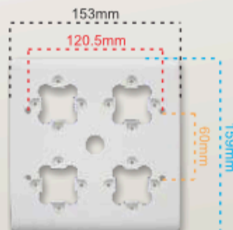
COVER FRAME FOR 4 MODULE SUITABLE FOR 5"X5" FRAME
